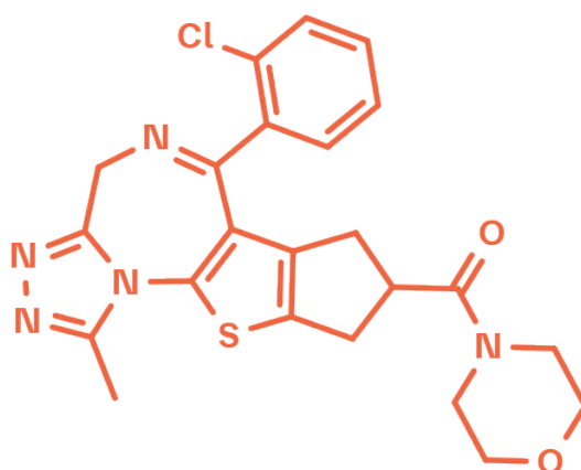
Figure 1: 2D structure of Bepafant
