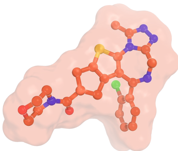
Figure 2: Bepafant, 3D conformation
