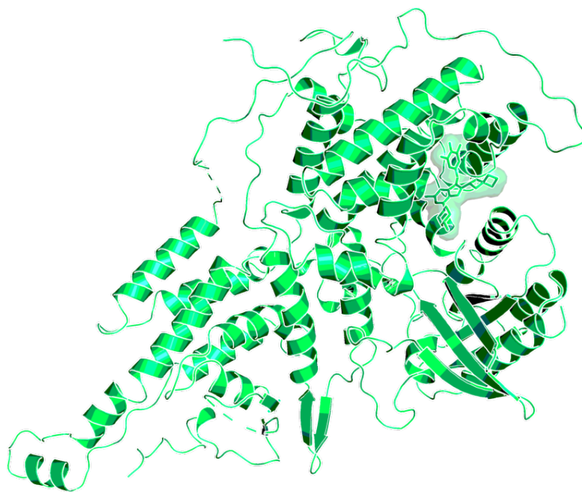
Figure 3: X-ray crystal structure of a complex including HRAS, SOS1, and VUBI1 (PDB code: 6D55)
