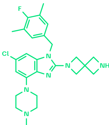
Figure 1: 2D structure of VUBI1 a SOS1 activator
