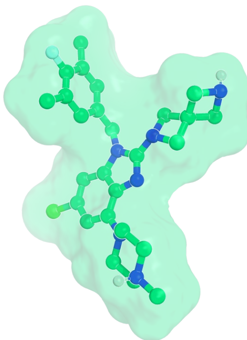
Figure 2: VUBI1, 3D conformation
