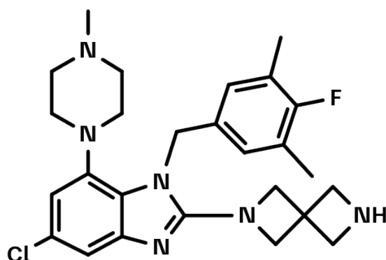
Figure 4: BI-9930 which serves as a negative control.
