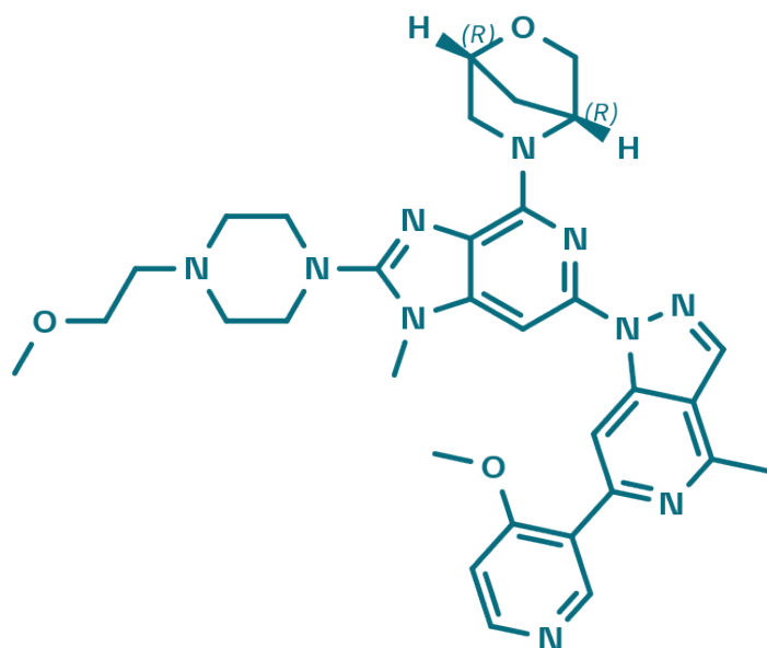
Figure 1: 2D structure of BI-8128, an orally bioavailable EGFR 4 th generation inhibitor
